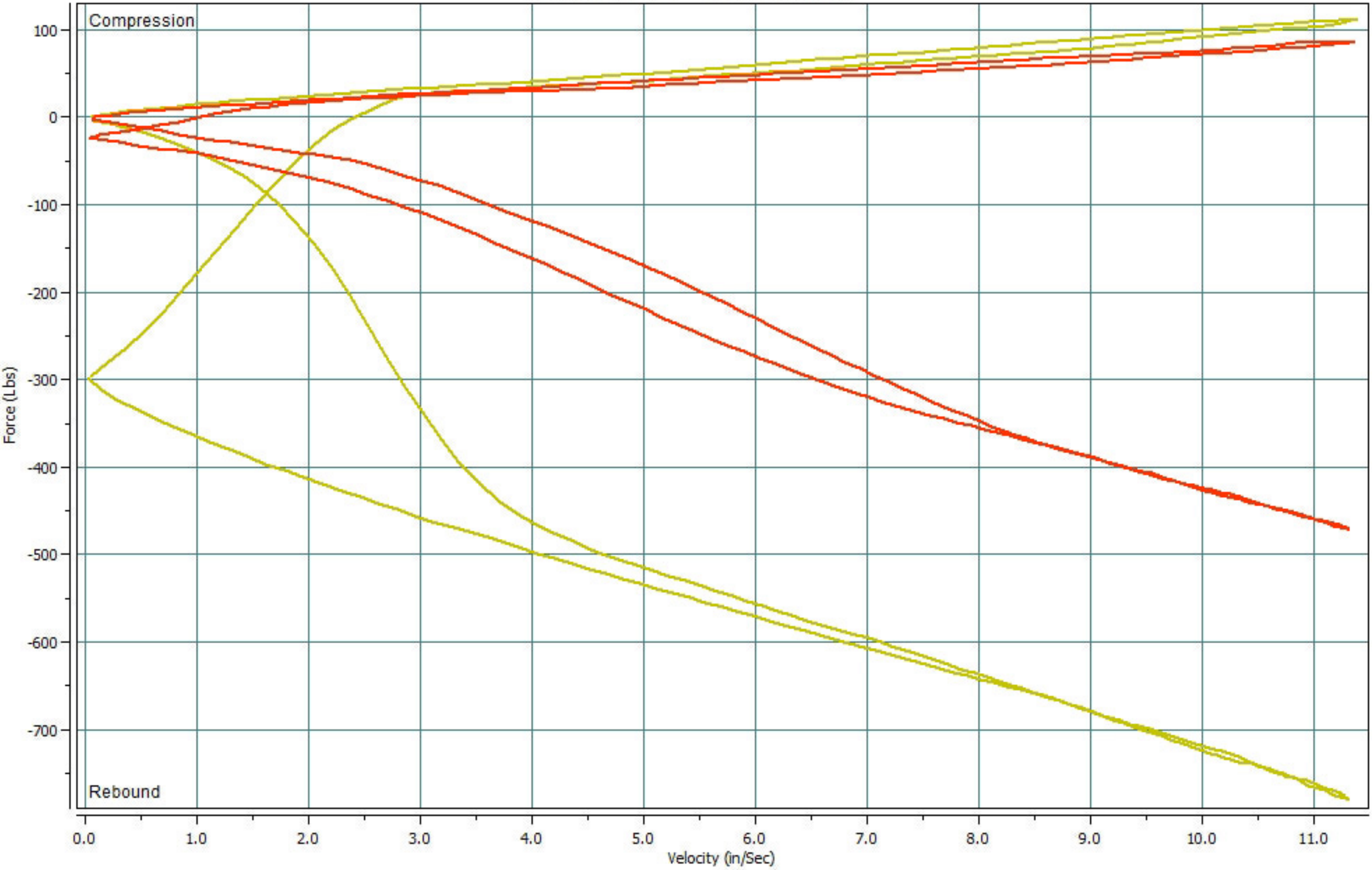
Force vs. Absolute Velocity BSB 2018 GF 300 ^ Shock 24395 2STAGE 300 GF Temp: 72.0 degF Rod Pressure: 39.5 Gas Pressure: 100
